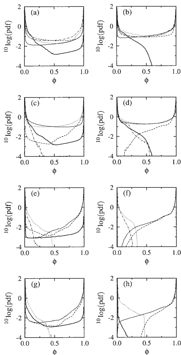
Figure 10. Concentration PDF of reactants and products over the cross-section at a close (a, c, e, g) and far (b, d, f, h) downstream position for a large (a, b, e, f) and small (c, d, g, h) Damköhler number and a high (a–d) and low (e–h) inlet concentration, with values \phi_{s0} - x/D_t - {}^{10}\log Da : (a) 4,000 – 0.0 – 3.7; (b) 4,000 – 4.75 – 3.7; (c) 4,000 – 0.0 – –4.3; (d) 4,000 – 4.75 – –4.3; (e) 1.0 – 0.0 – 3.9; (f) 1.0 – 4.75 – 3.9; (g) 1.0 – 0.0 – –4.1; (h) 1.0 – 4.75 – –4.1.
