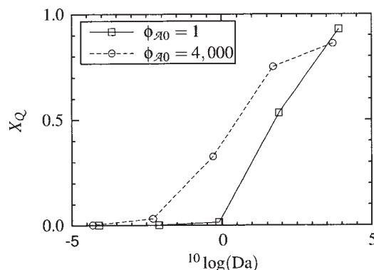
Figure 12. Final yield vs. Damköhler number for low and high inlet concentration of \mathcal{A} .
